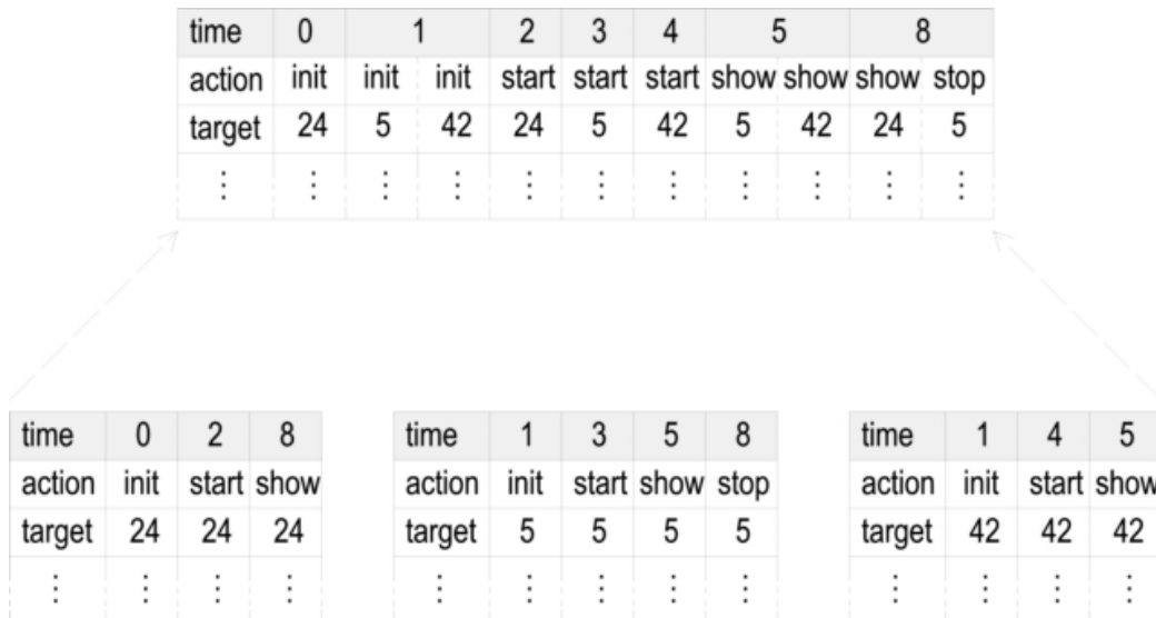
Figure 3: : Playlists under Linearisation
