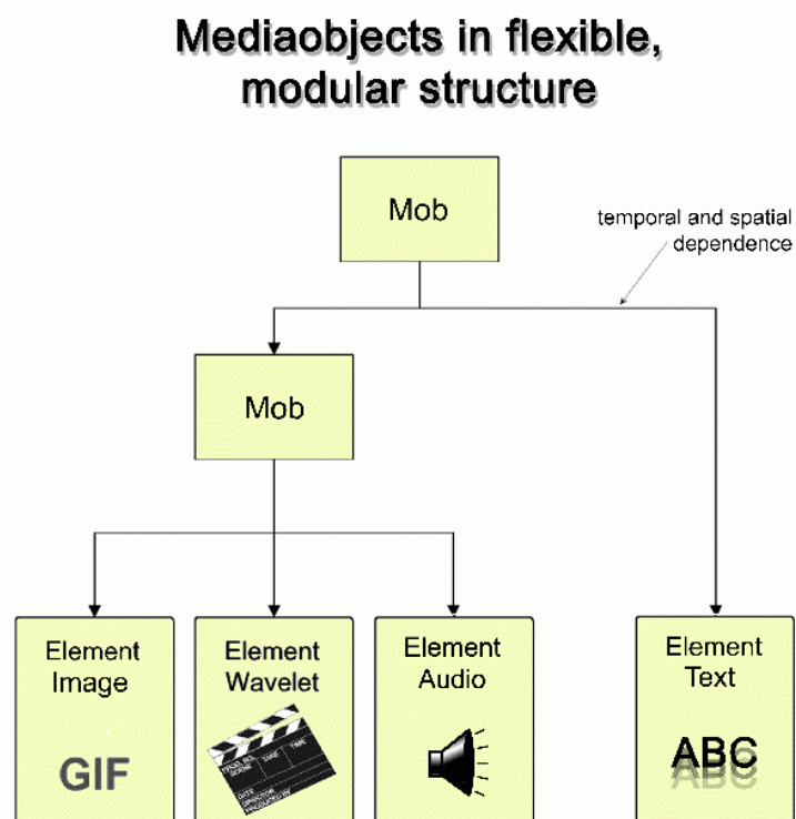
Figure 2: Media Object Hierarchy
