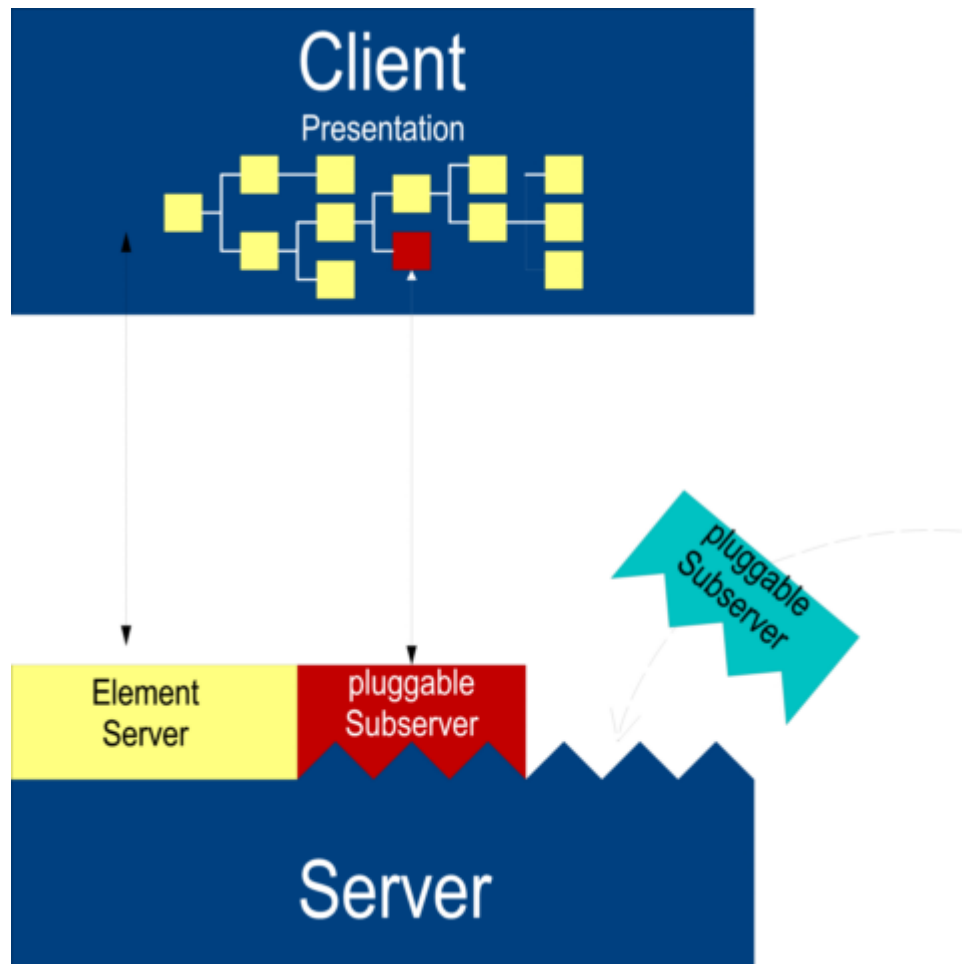
Figure 5: Sub server Extensions
