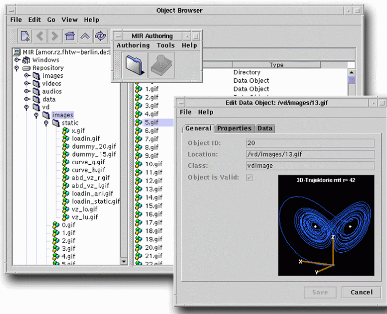
Figure 6: Authoring Media from the Web
